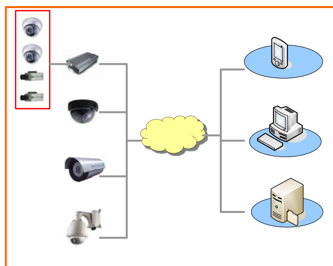
IP CAMERA - Connection Structure diagram
